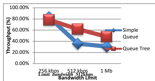
Gambar 8. Grafik Perbandingan Throughput
